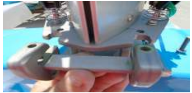
Mast raising bracket ready to be installed
