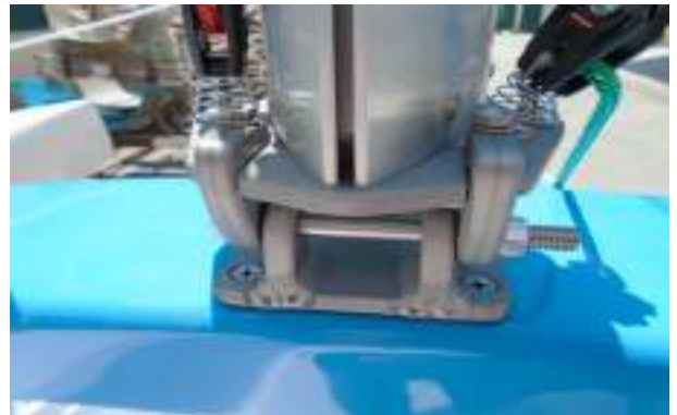
Mast raising bracket after installation to mast base
