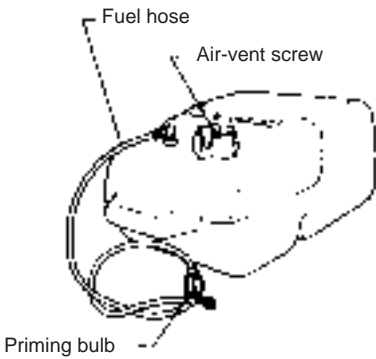
FUEL TANK
